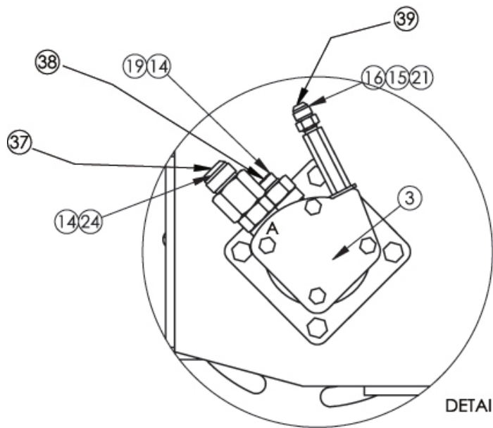
DETAIL C
